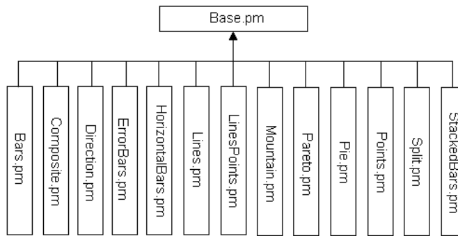
Figure 1: The hierarchy of Chart classes
