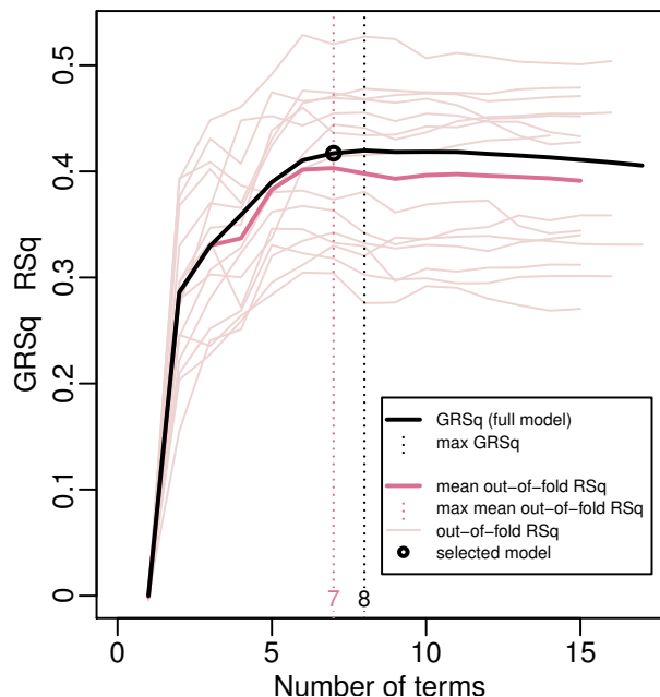
Figure 18: Selecting a model with pmethod="cv" .
